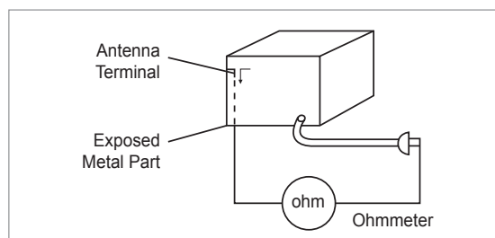
<Fig. 1-2 Insulation Resistance Test>
